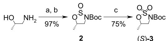
Scheme 1. Reagents and conditions: (a) (Boc) 2 O, CH 2 Cl 2 ; (b) SOCl 2 , imidazole, CH 2 Cl 2 , –50 °C; (c) NaIO 4 , RuO 2 , EtOAc.
