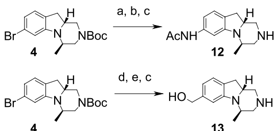
Scheme 4. Reagents and conditions: (a) Pd 2 (dba) 3 , (±)-BINAP, NaOt-Bu, toluene, benzophenone imine; Pd/C, NH 4 -formate, MeOH; (b) AcCl, NEt 3 , CH 2 Cl 2 ; (c) TFA, CH 2 Cl 2 ; (d) n -BuLi, THF, CO 2 , –78 °C; (e) LiAlH 4 , THF.
